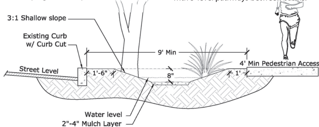
Figure 4. Typical cross-section of a basin with sloping sides, showing typical setbacks for a site on a residential street with on-street parking. For plan view see Appendix.
