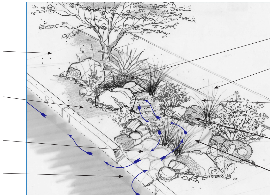
Figure 3. Conceptual drawing of a curb cut and rock-lined basin in the ROW.
