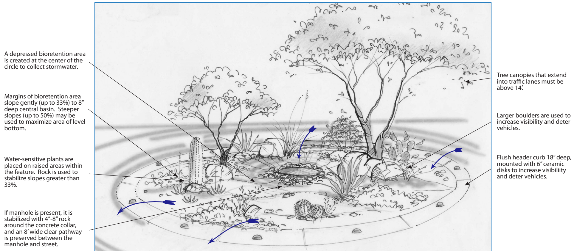
Figure 13. Conceptual drawing of a traffic circle with depressed bioretention area for a neighborhood street.
