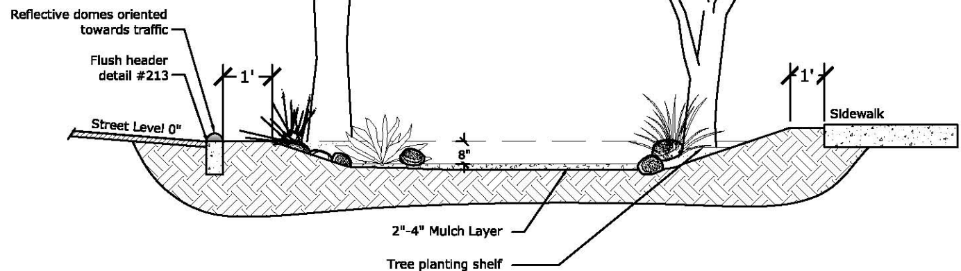
Figure 14. Typical cross-section of a street width reduction with flush curbs and depressed bioretention area. For plan view, see Appendix.
