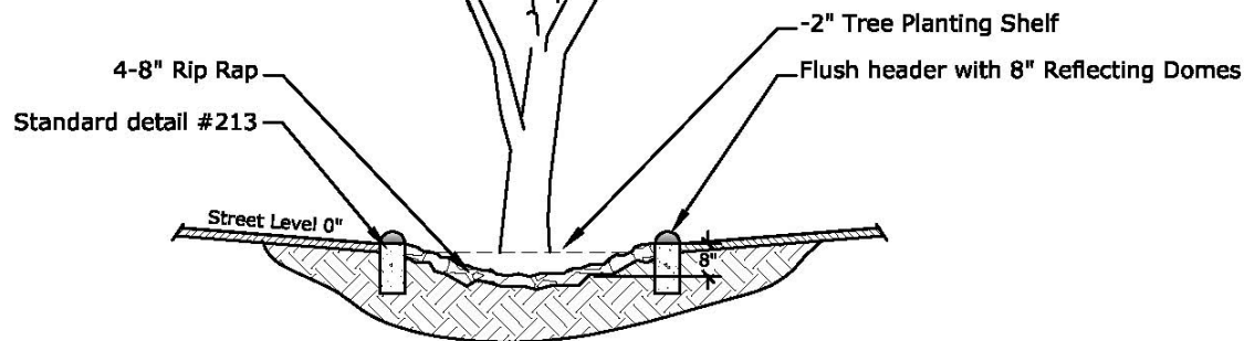
Figure 10. Typical cross-section of a median with flush curbs and depressed bioretention area. For plan view, see Appendix.
