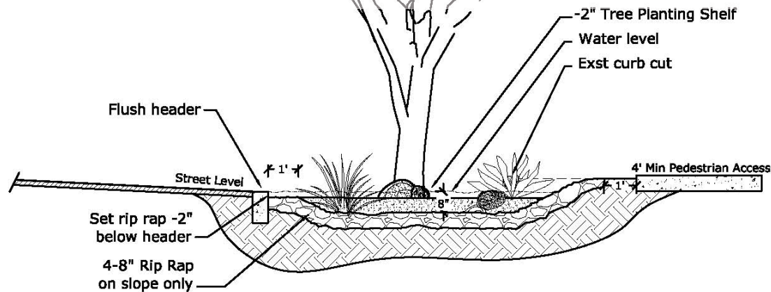
Figure 8. Typical cross-section of a chicane with flush curb and depressed bioretention area. For plan view, see Appendix.
