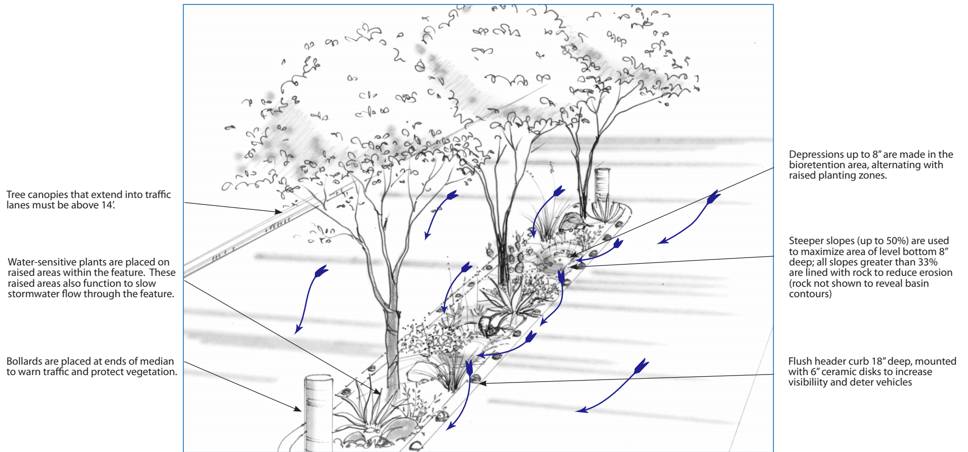
Figure 11. Conceptual drawing of a median with depressed bioretention area for a neighborhood street.
