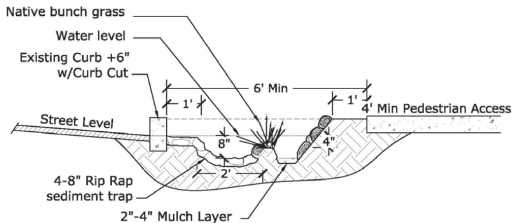
Figure 6. Typical cross section of sediment trap for curb cut with rock-lined basin.
