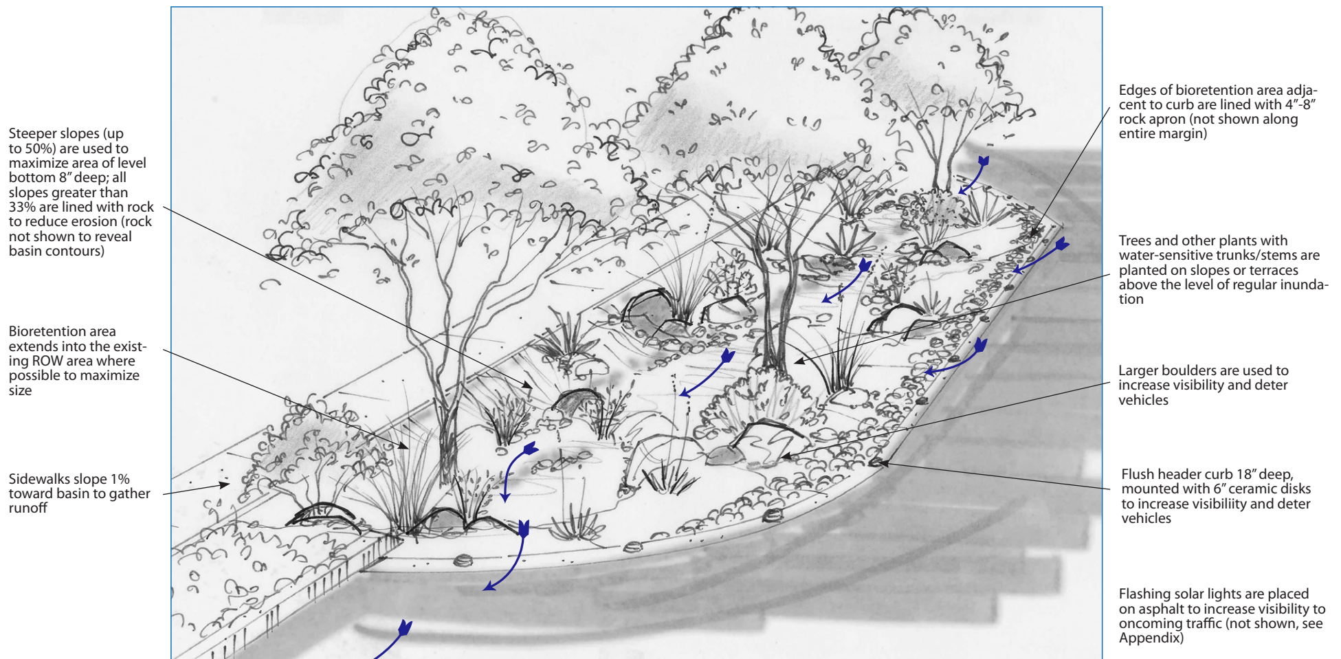
Figure 15. Conceptual drawing of a street width reduction with depressed bioretention area for a neighborhood street.
