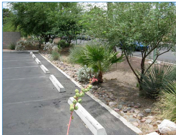
A bioretention basin captures and filters stormwater from a restaurant parking lot and the street.
