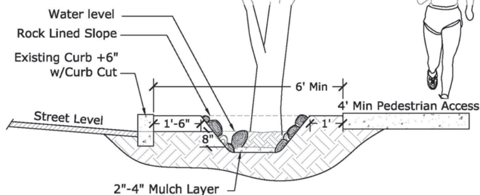
Figure 2. Typical cross-section of a basin with rock-lined edges, showing typical setbacks for a site on a residential street with on-street parking (for plan view see Appendix).
