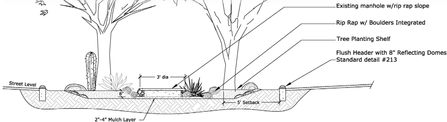
Figure 12. Typical cross-section of a traffic circle with flush curbs and depressed bioretention area. For plan view, see Appendix.
